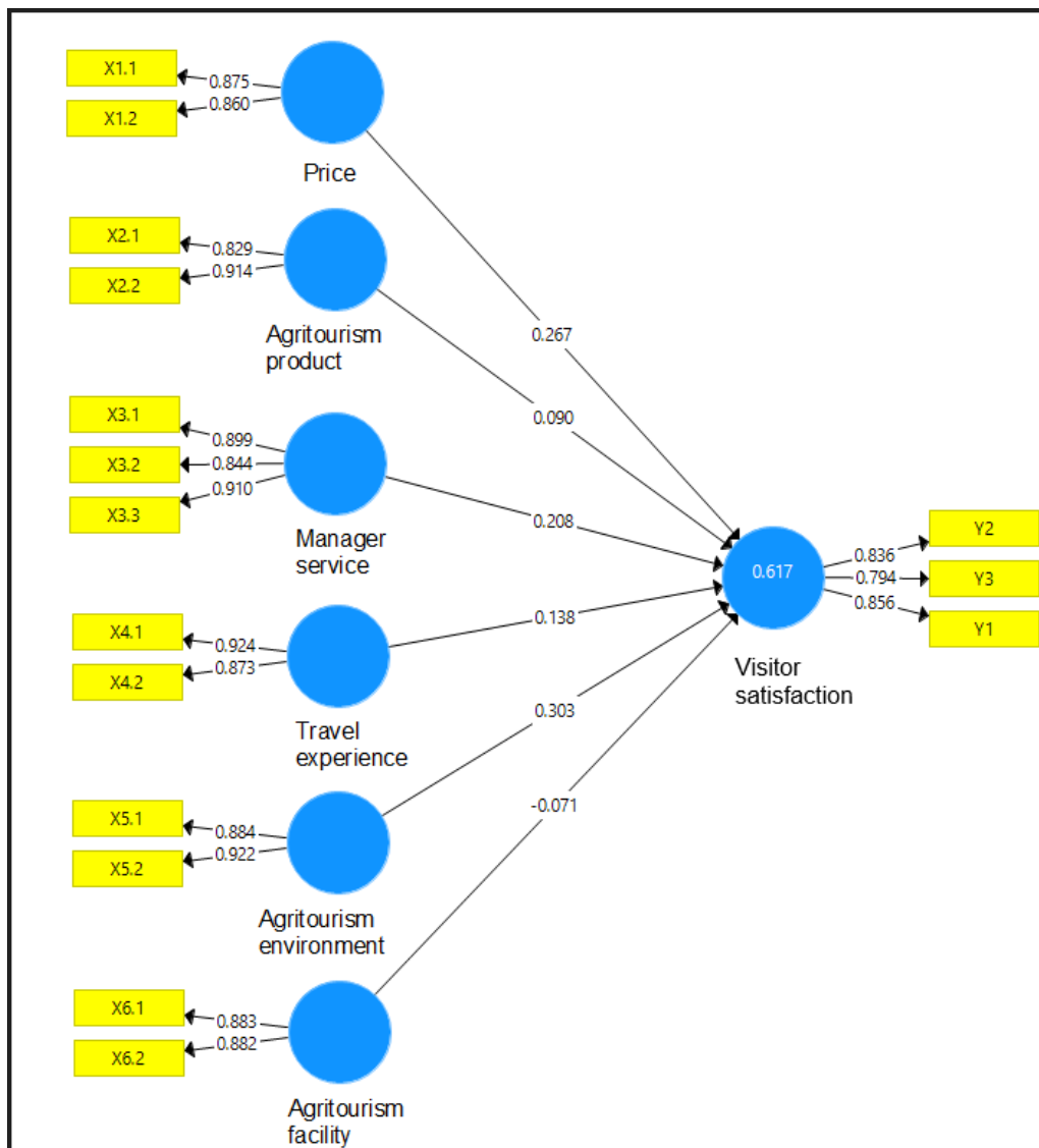
Fig. 1. Measurement model
