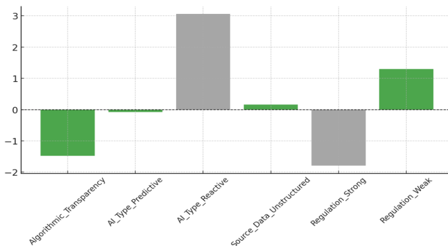
Fig. 4. Regression coefficients
