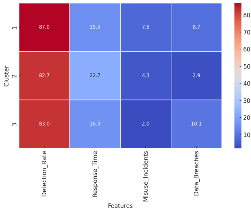
Fig. 7. Cluster centroids
